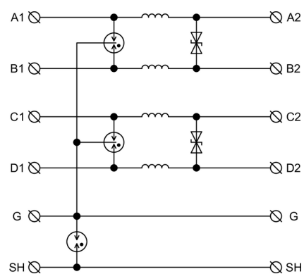
Internal diagram
