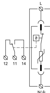
Internal diagram
