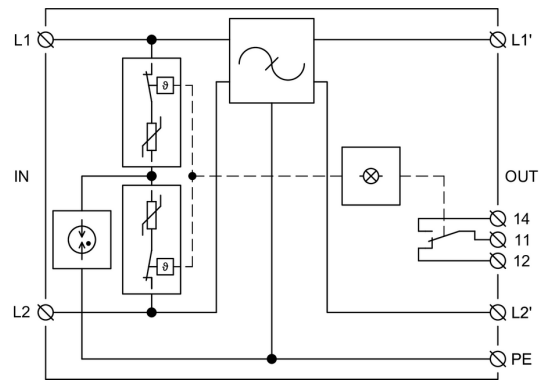
Internal diagram
