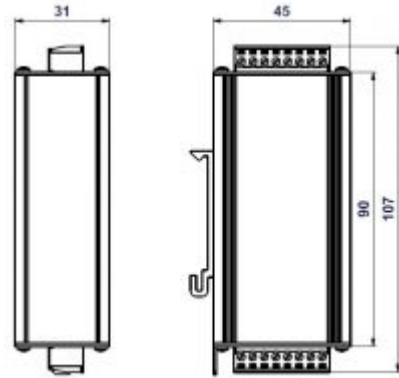
Dimension drawing
