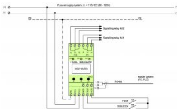
Installation diagram
