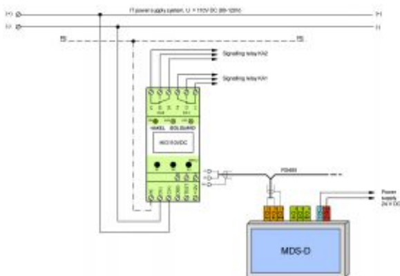
Installation diagram
